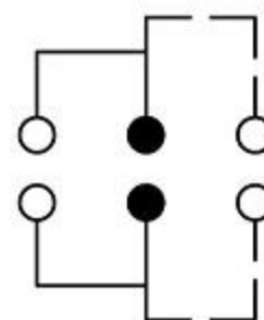
SCHEMATIC (NON-SHORTING)
